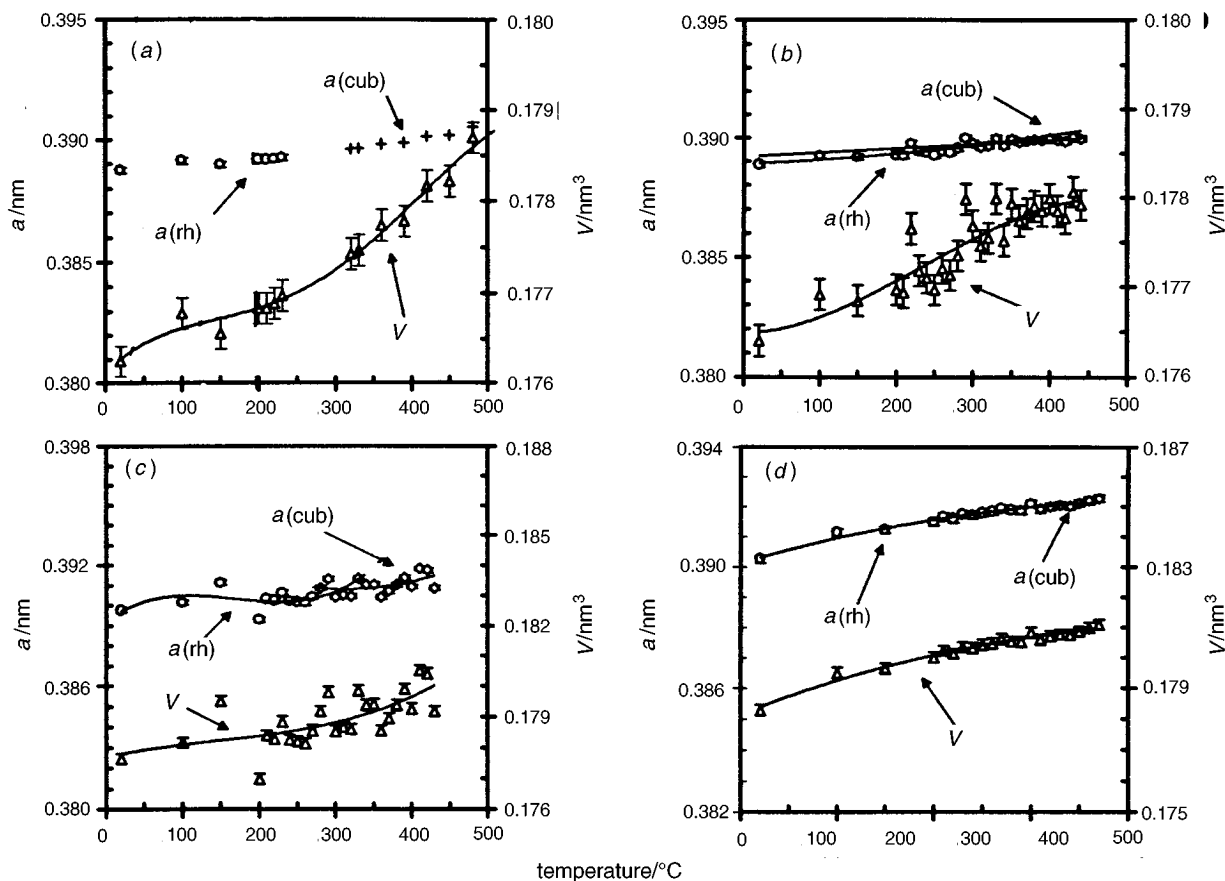
Fig. 2 NBT-PT system: rhombohedral range. Lattice parameters and cell volume vs. temperature for (\text{Na}_{0.5}\text{Bi}_{0.5})_{1-x}\text{Pb}_x\text{TiO}_3 : x=0 (a), 0.03 (b), 0.05 (c) and 0.09 (d).
