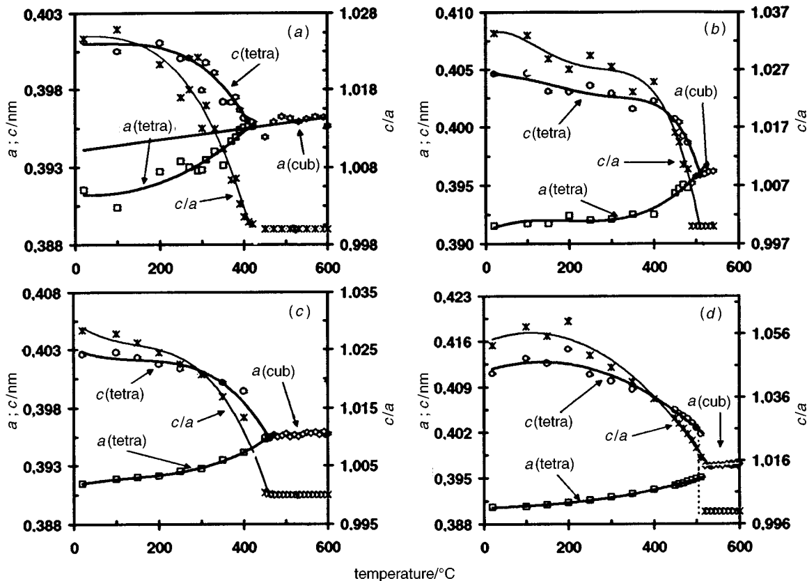
Fig. 5 KBT-PT system. Lattice parameters vs. temperature for (\text{K}_{0.5}\text{Bi}_{0.5})_{1-x}\text{Pb}_x\text{TiO}_3 : x=0.05 (a), 0.20 (b), 0.40 (c) and 0.90 (d).
