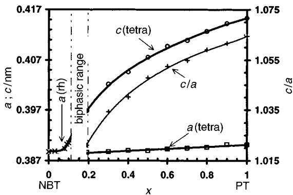
Fig. 1 NBT-PT system. Room-temperature lattice parameters vs. composition.
