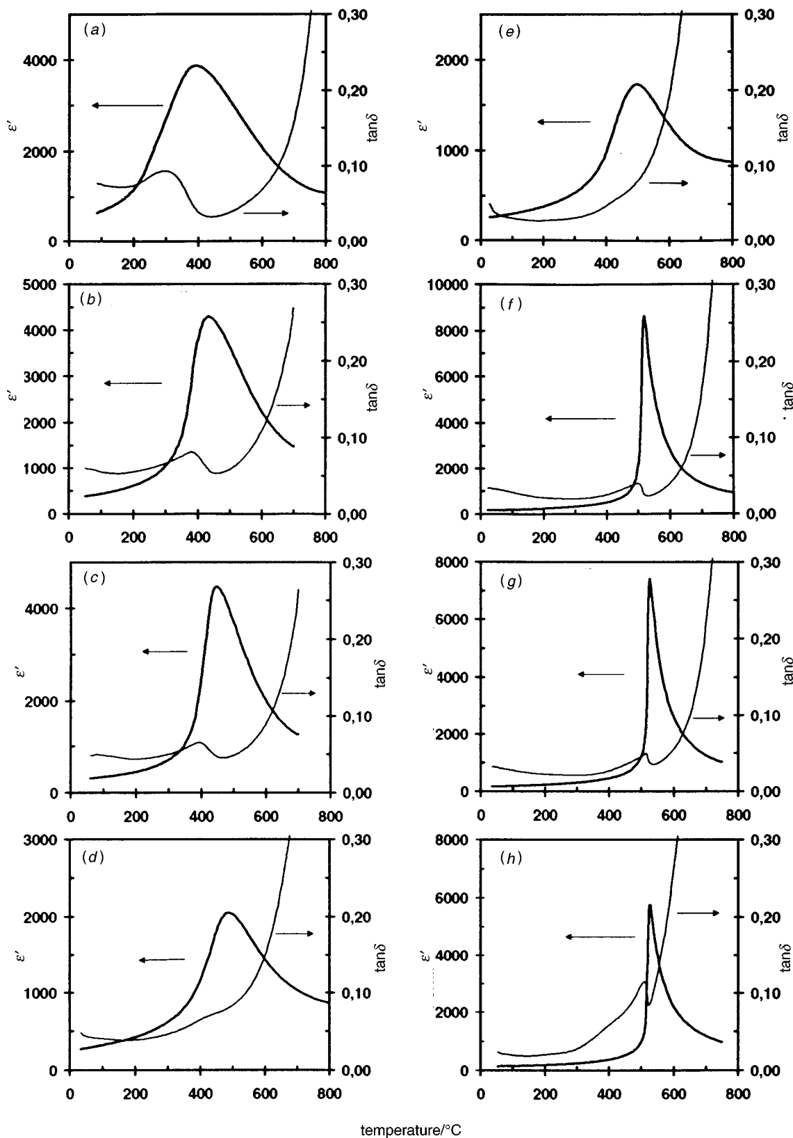
Fig. 7 KBT-PT system. Permittivity and loss vs. temperature for (\text{K}_{0.5}\text{Bi}_{0.5})_{0.51-x}\text{Pb}_x\text{TiO}_3 : x=0 (a), 0.09 (b), 0.18 (c), 0.30 (d), 0.40 (e), 0.50 (f), 0.60 (g) and 0.80 (h).
