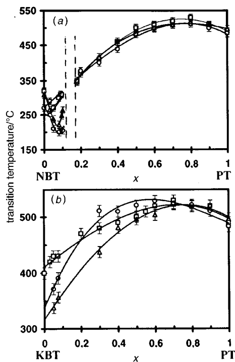
Fig. 9 Transition temperatures vs. composition from HTXRD ( \square , increasing T ) and DSC ( \Delta , increasing T ; \circ , decreasing T ) for (a) NBT-PT and (b) KBT-PT
