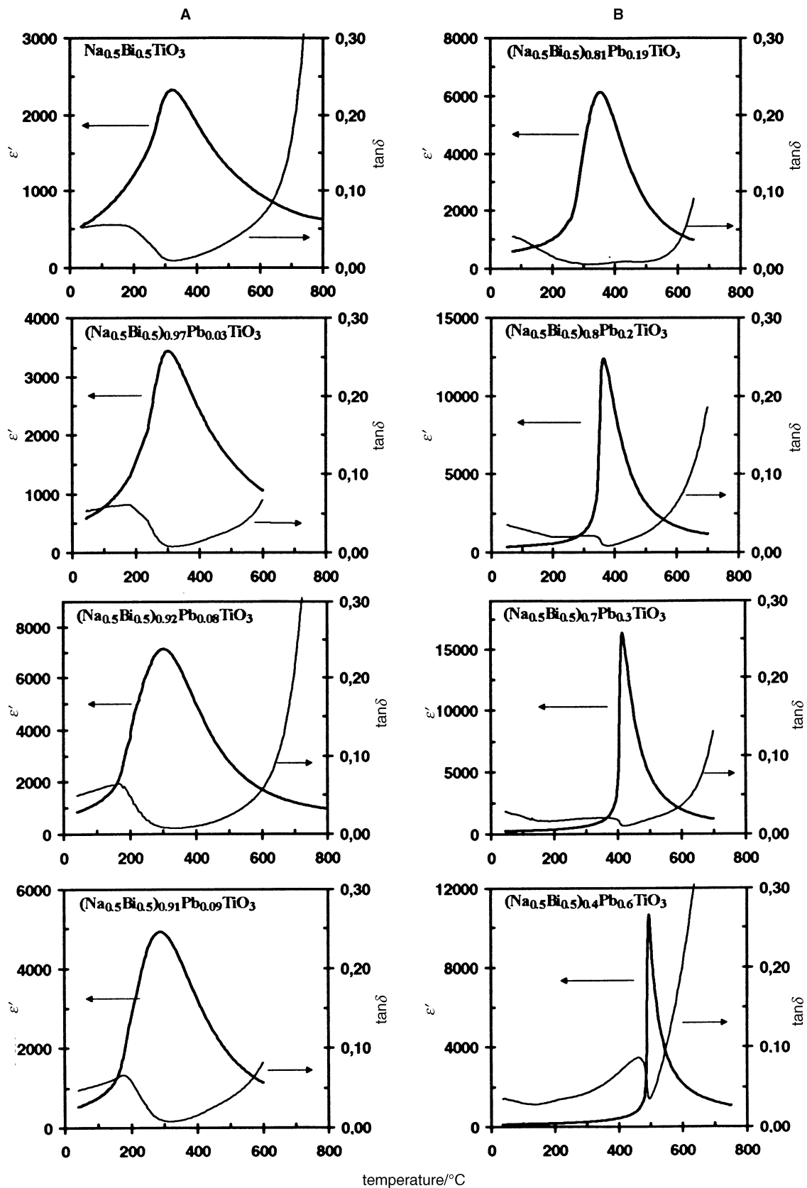
Fig. 6 NBT-PT system. Permittivity and loss vs. temperature for (\text{Na}_{0.5}\text{Bi}_{0.5})_{1-x}\text{Pb}_x\text{TiO}_3 . A, rhombohedral range: x=0 (a), 0.03 (b), 0.08 (c) and 0.09 (d). B, tetragonal range: x=0.19 (a), 0.20 (b), 0.30 (c) and 0.60 (d).
