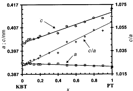
Fig. 4 KBT-PT system. Room-temperature lattice parameters vs. composition.
